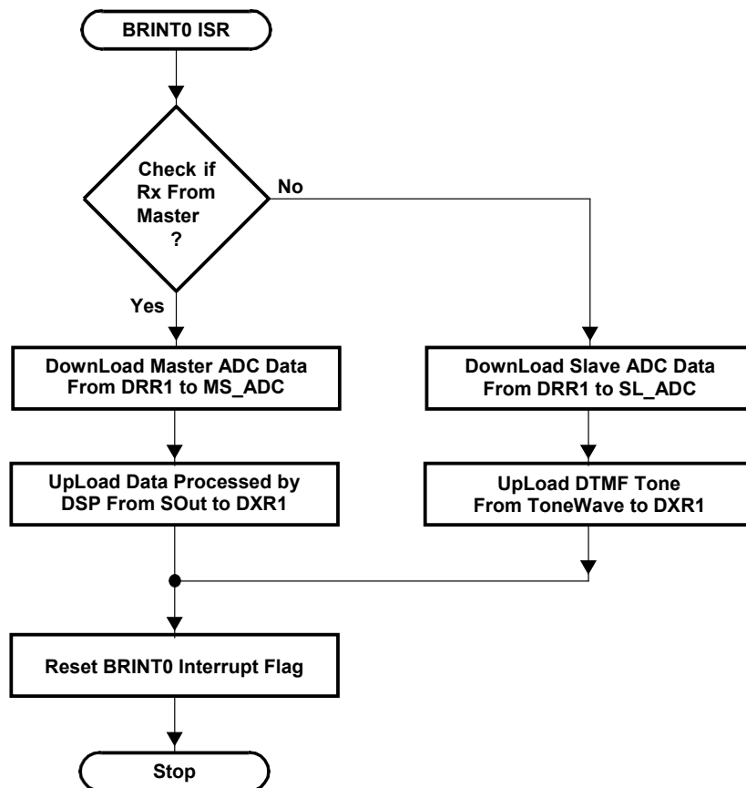
Figure 9. BRINIT ISR Flow Chart
