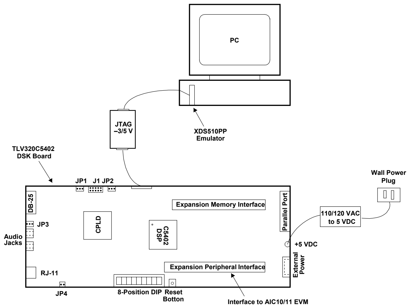
Figure 2. System Connection
