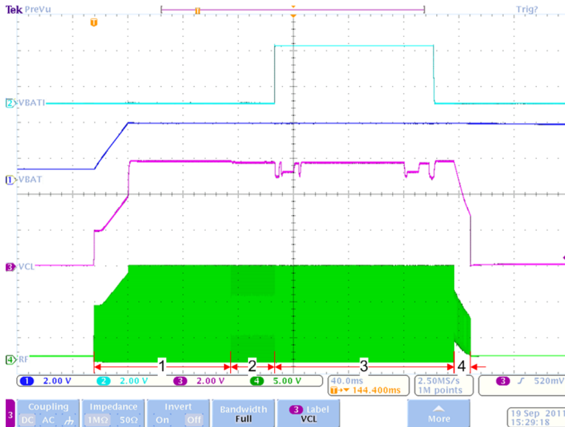
Figure 12. Overview of Complete Telegram
