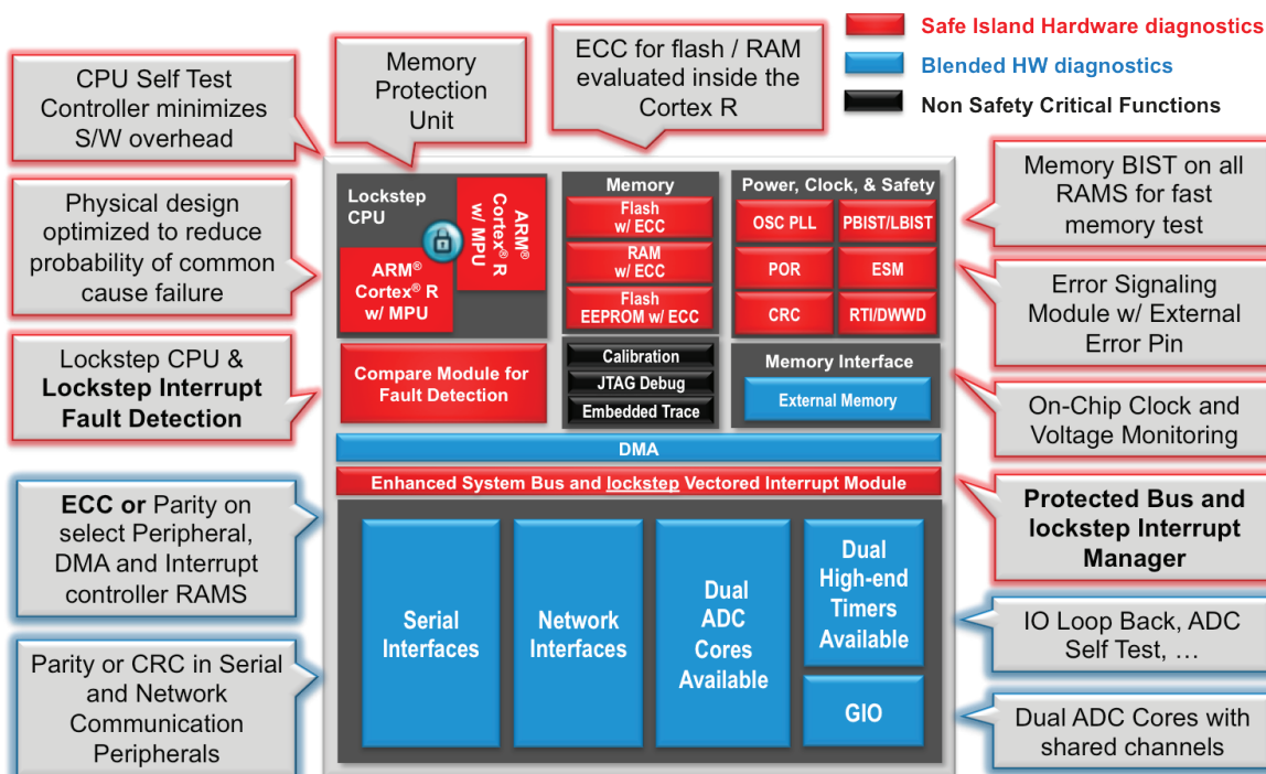
Figure 7: Hercules MCU safety features
