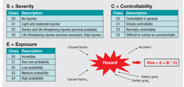
Figure 4: ISO 26262 hazard analysis and risk assessment
