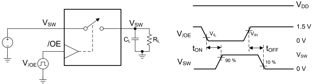
Figure 7-5. t_{ON} and t_{OFF} Timing for \overline{OE}
