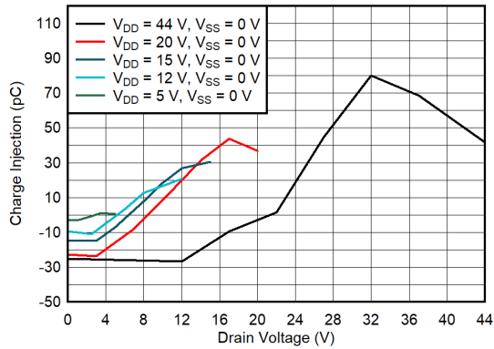
Figure 6-15. Charge Injection vs Drain Voltage – Single Supply
