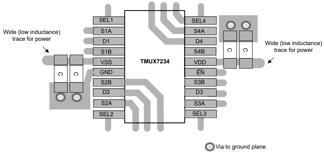
Figure 11-2. TMUX7234 Layout Example
