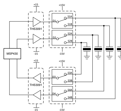
Figure 3-1. Application Diagram
