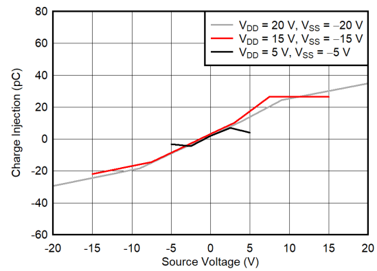
Figure 6-12. Charge Injection vs Source Voltage – Dual Supply
