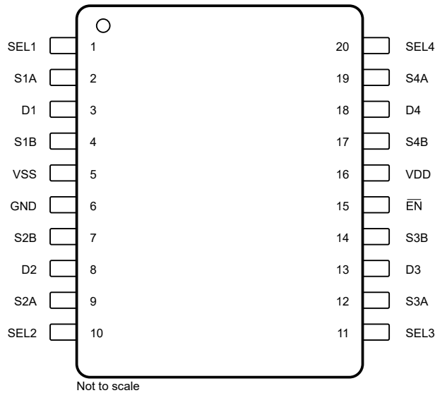
Figure 5-1. TMUX7234 PW Package 20-Pin TSSOP (Preview) Top View
