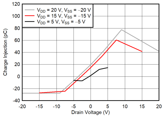
Figure 6-13. Charge Injection vs Drain Voltage – Dual Supply
