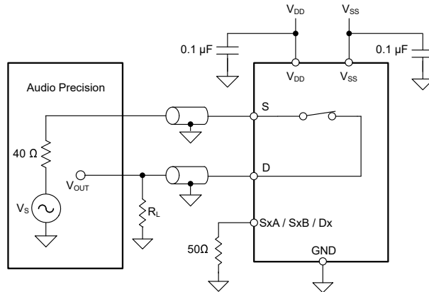
Figure 7-13. THD+N Measurement Setup
