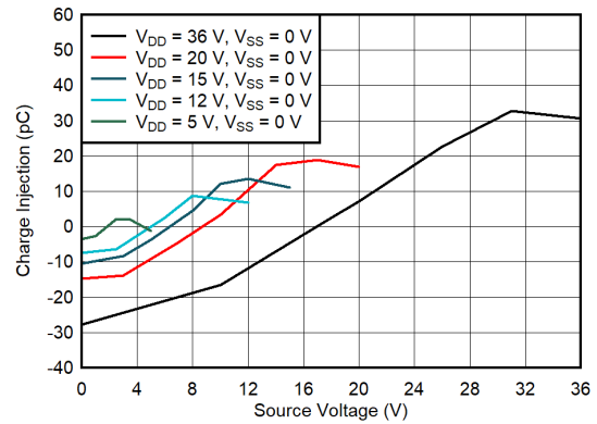
Figure 6-14. Charge Injection vs Source Voltage – Single Supply
