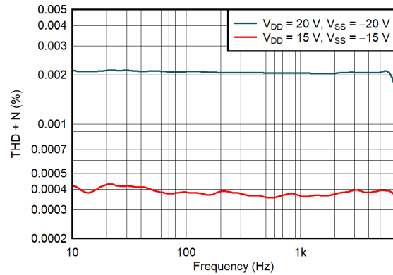
Figure 6-22. THD+N vs Frequency (Dual Supply)
