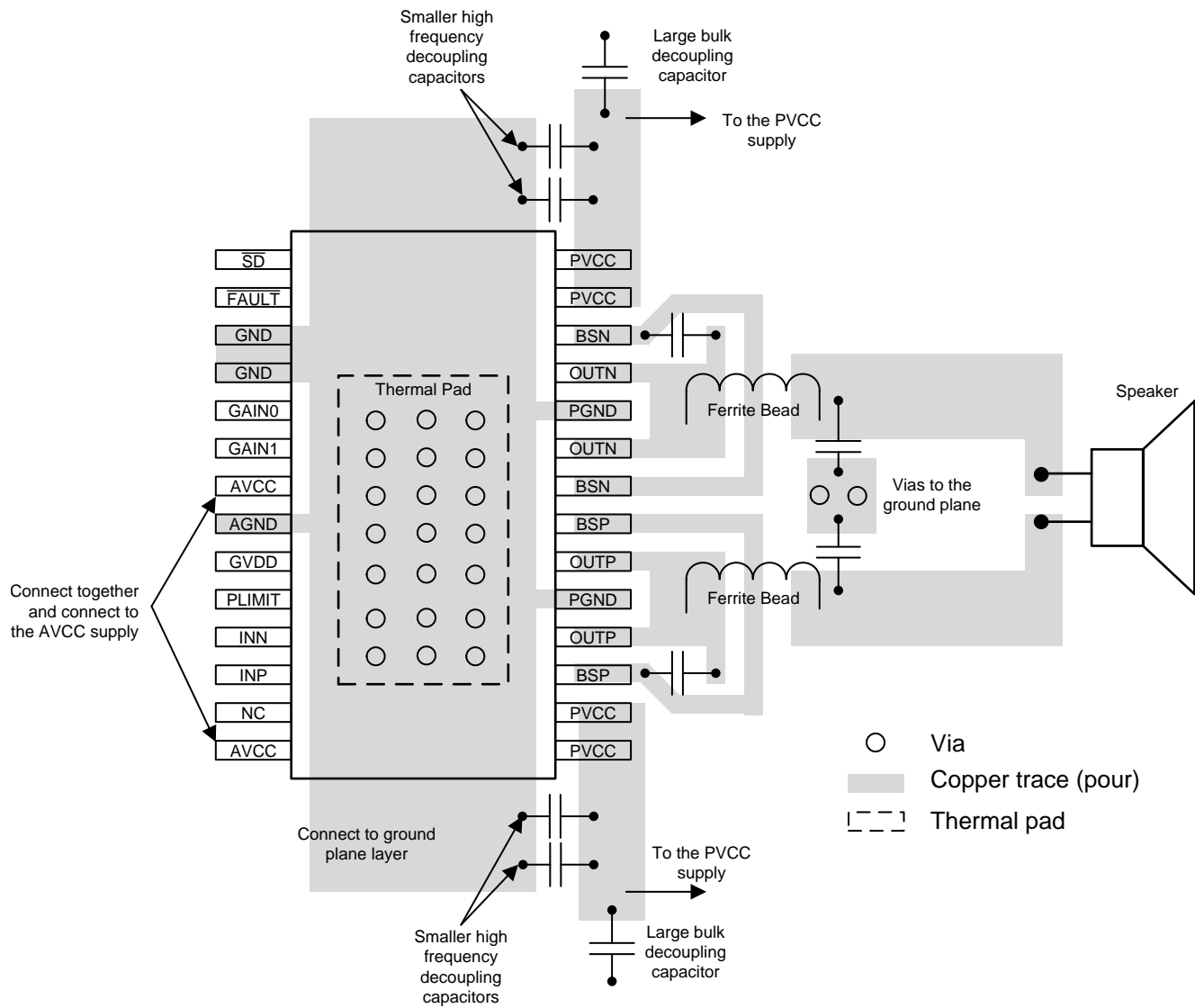
Figure 21. Recommended Layout
