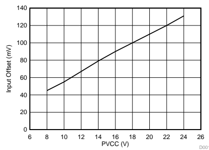
Figure 1. DC Detect Threshold at Input Versus PVCC
