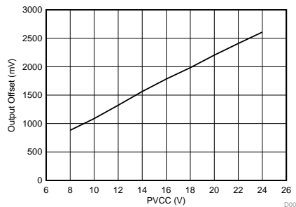
Figure 2. DC detect threshold at output Versus PVCC
