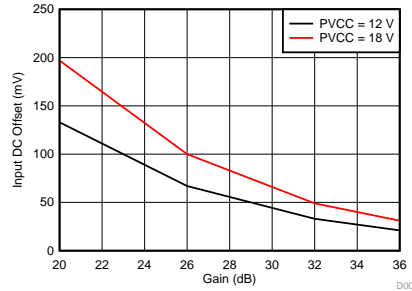
Figure 3. DC Detect Threshold at Input Versus Gain
