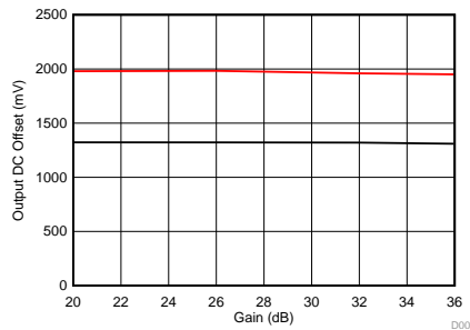
Figure 4. DC Detect Threshold at Output Versus Gain
