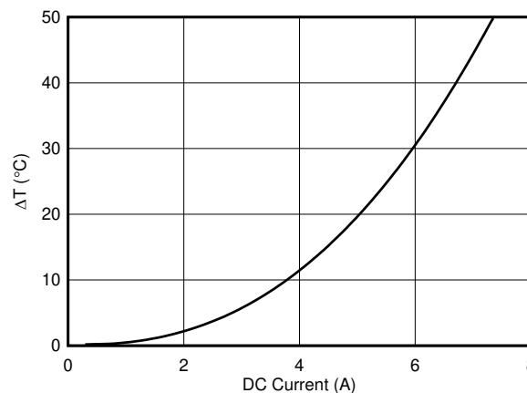
Figure 4. Temperature Rise vs DC Current
