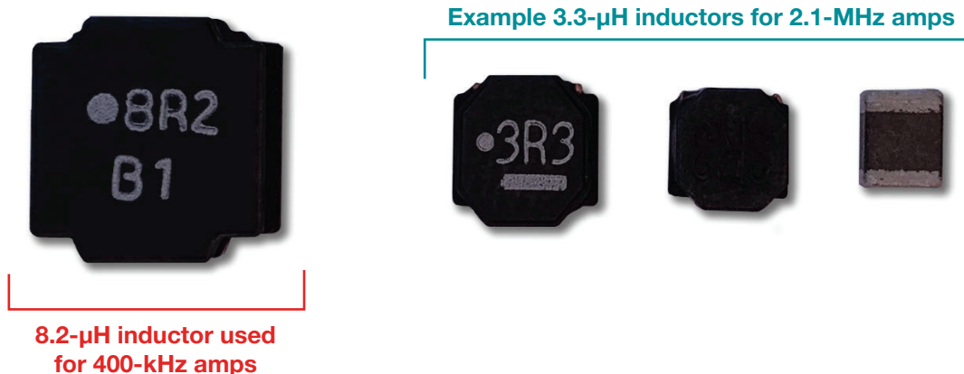
Figure 5. Comparison of inductor size vs. switching frequency.
