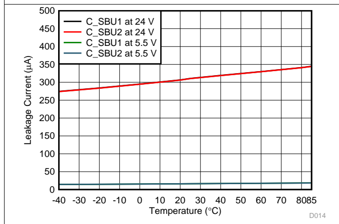
Figure 9. C_SBU OVP Leakage Current vs Ambient Temperature at 5.5 V and 24 V
