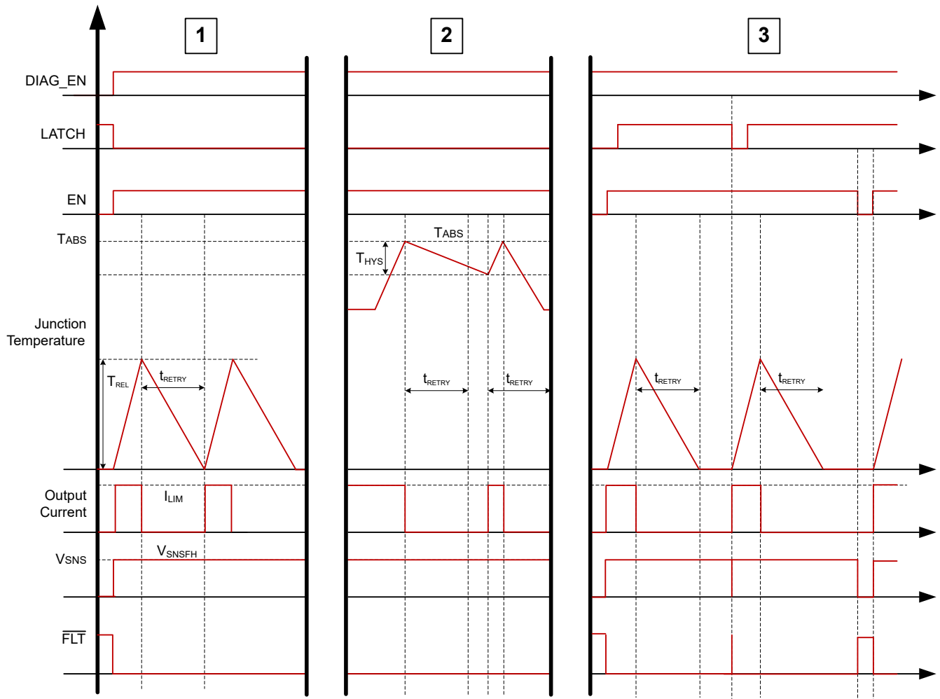
Figure 8-14. Thermal Behavior
