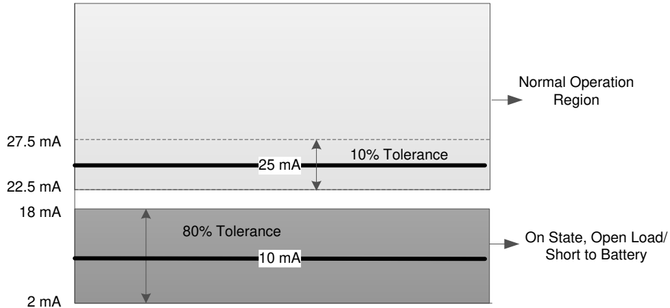
Figure 8-11. On-State Open-Load Detection and Normal-Operation Diagram
