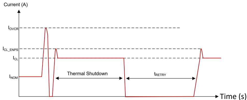
Figure 8-9. On-State Short-Circuit Behavior
