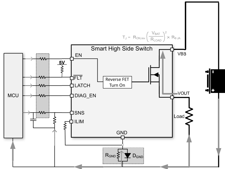
Figure 8-19. Reverse Protection with GND Network
