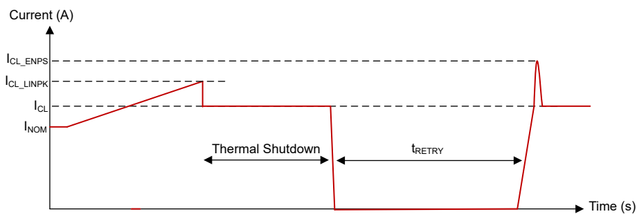
Figure 8-10. Overload Behavior
