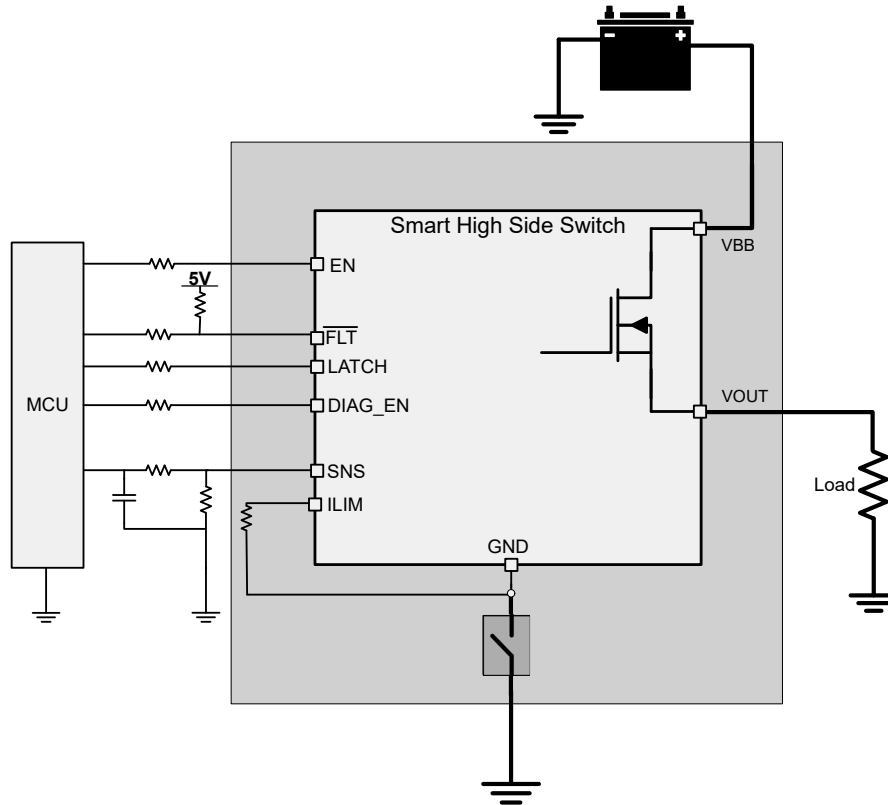
Figure 8-15. Loss of Device GND
