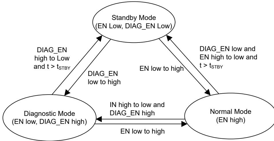
Figure 8-21. Work Mode State Machine
