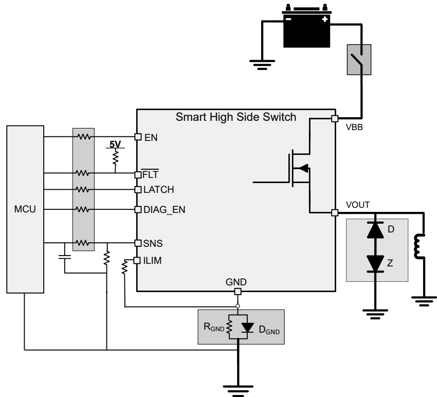
Figure 8-17. Loss of Battery
