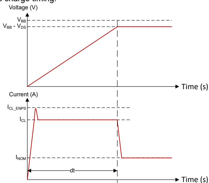
Figure 8-5. Capacitive Charging Timing
