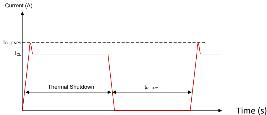
Figure 8-8. Enable into Short-Circuit Behavior (LATCH=0)
