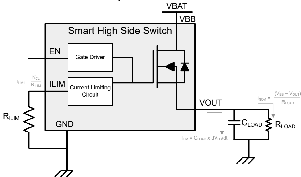
Figure 8-4. Capacitive Charging Circuit
