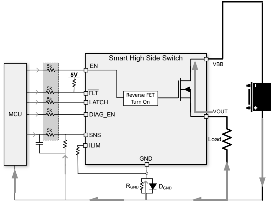
Figure 8-20. MCU I/O Protections
