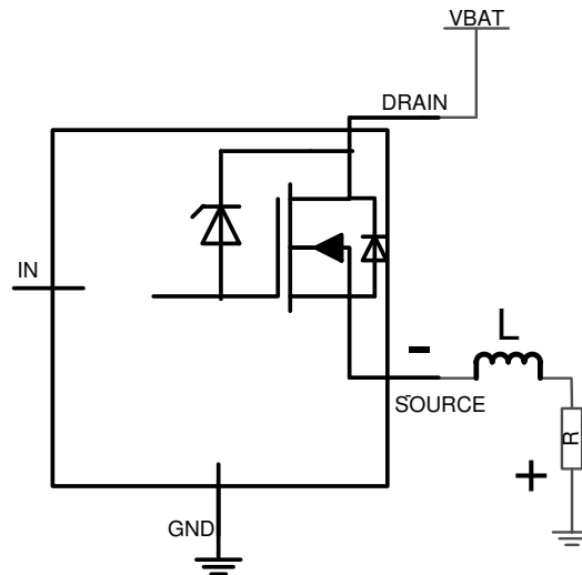
Figure 8-6. Driving Inductive Load
