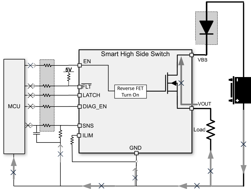
Figure 8-18. Reverse Protection with Blocking Diode
