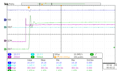
Current Limit Application
