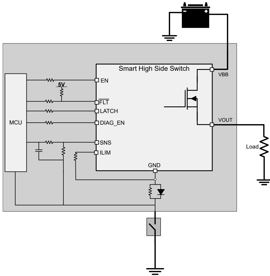
Figure 8-16. Loss of Module GND
