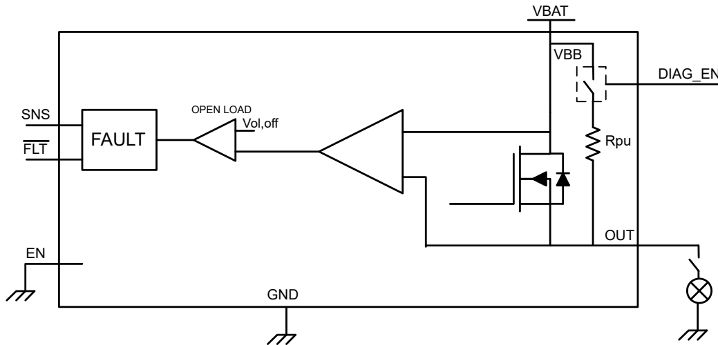
Figure 8-12. Open-Load Detection Circuit
