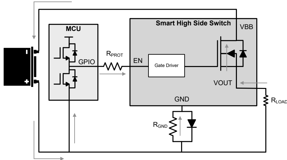
Figure 8-13. Reverse Battery Circuit
