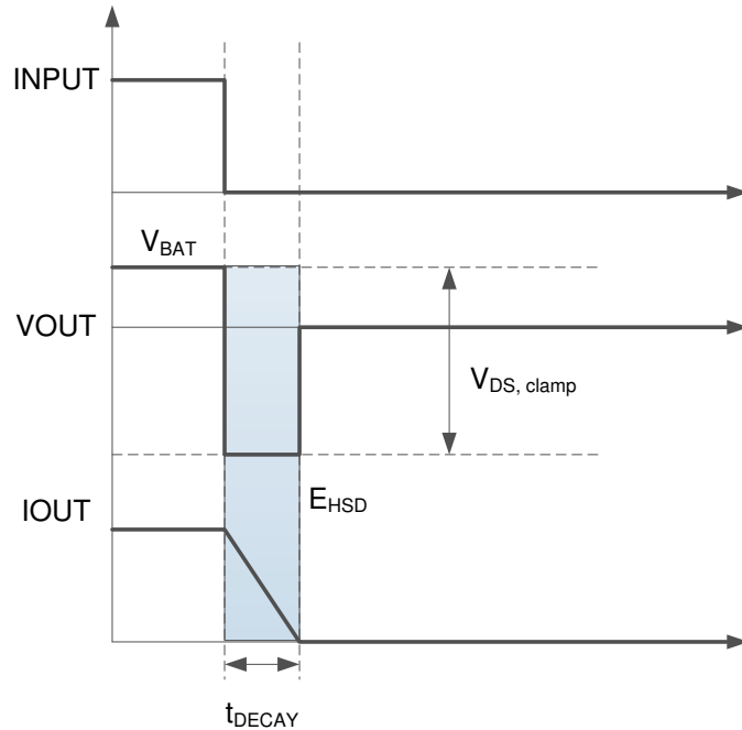
Figure 8-7. Inductive-Load Switching-Off Diagram
