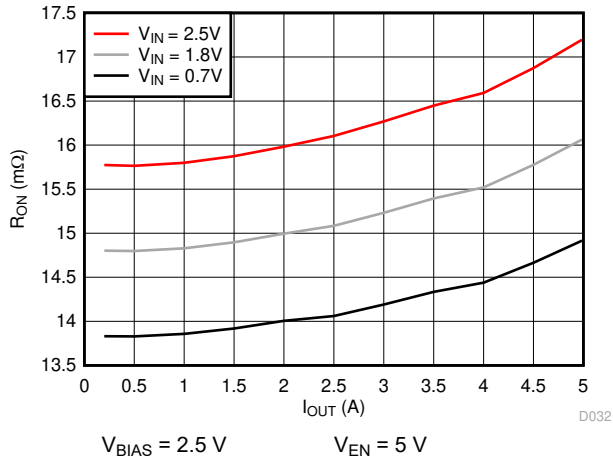
Figure 7-13. R_{ON} vs I_{OUT} , V_{BIAS} = 2.5 V
