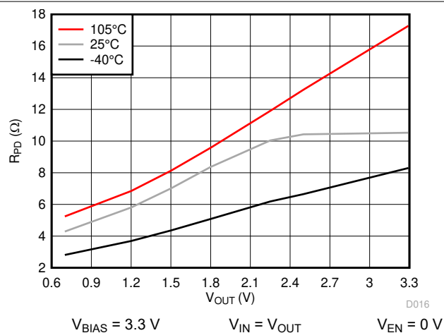
Figure 7-17. R_{PD} vs V_{OUT} , V_{BIAS} = 3.3 V
