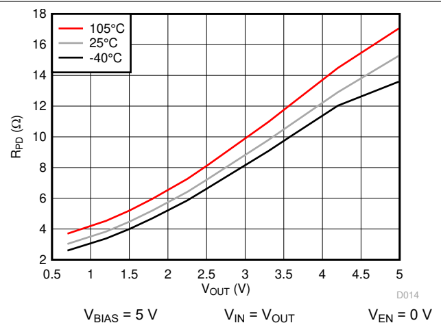
Figure 7-18. R_{PD} vs V_{OUT} , V_{BIAS} = 5 V
