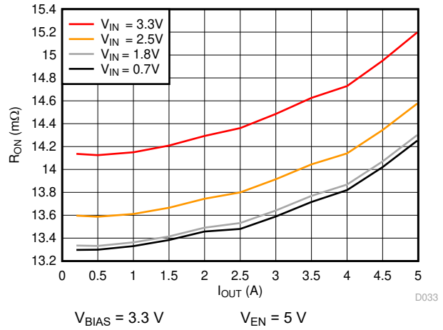
Figure 7-14. R_{ON} vs I_{OUT} , V_{BIAS} = 3.3 V
