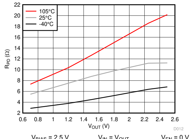
Figure 7-16. R_{PD} vs V_{OUT} , V_{BIAS} = 2.5 V
