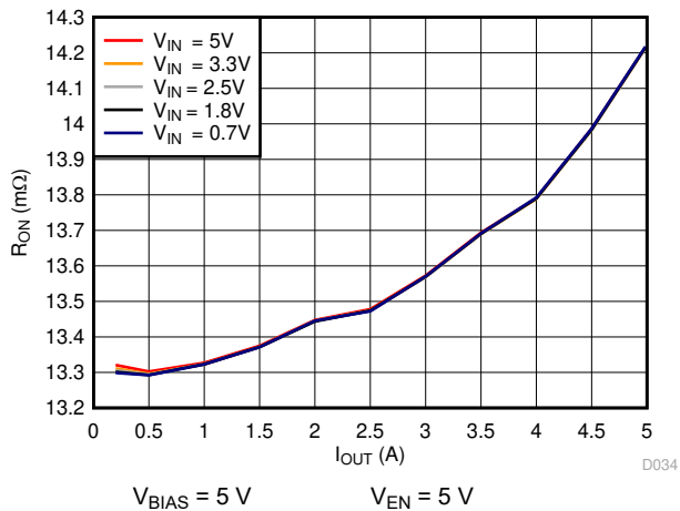
Figure 7-15. R_{ON} vs I_{OUT} , V_{BIAS} = 5 V
