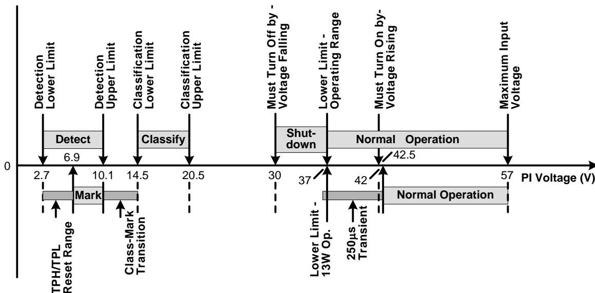
Figure 15. Operational States
