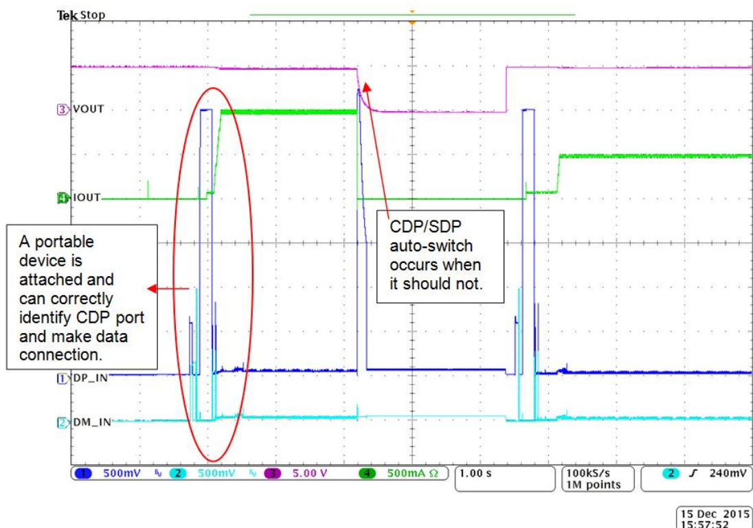
Figure 1. CDP/SDP Auto-Switch Occurs Incorrectly
