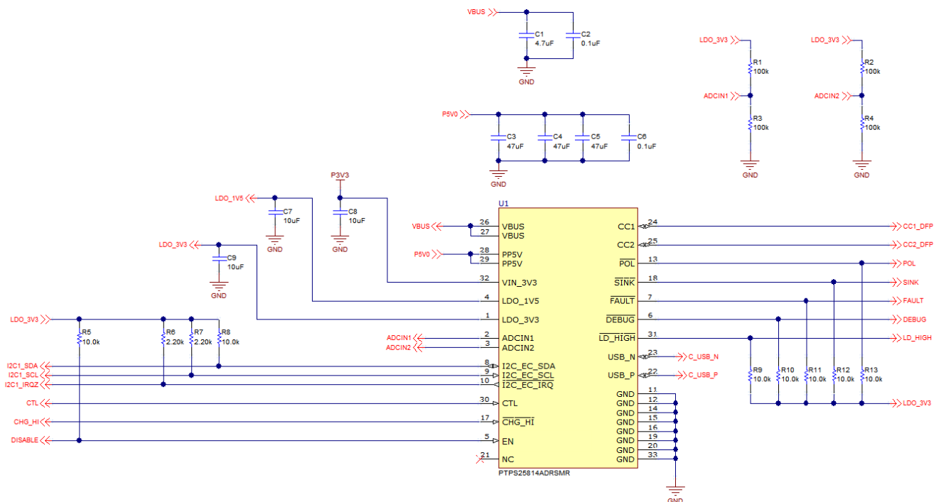
Figure 11-1. Example Schematic
