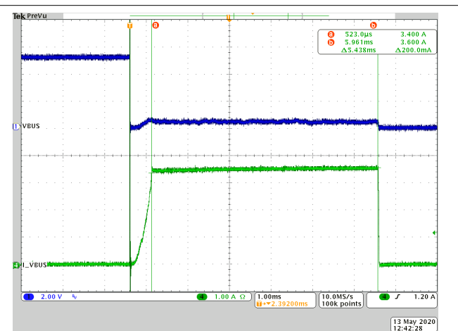
Figure 9-4. VBUS Short to Ground (Zoomed Out)
