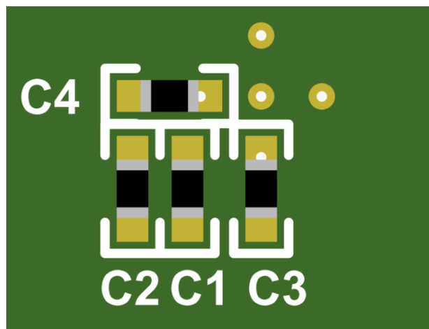
Figure 11-5. Bottom View 3-D
