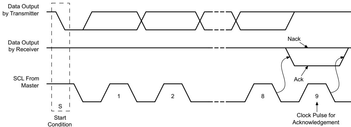
Figure 8-9. I 2 C Acknowledgment
