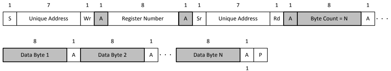
Figure 8-11. I 2 C Unique Address Read Register Protocol
