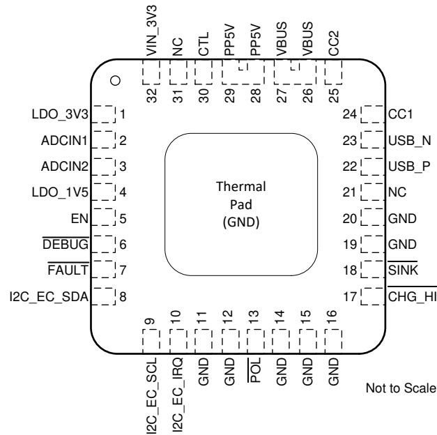
Figure 5-1. RSM Package 32-pin QFN Top View
