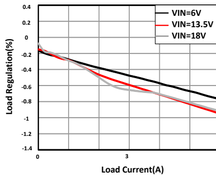
Figure 11-5. Load Regulation
