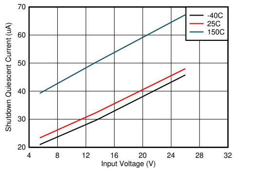
Figure 8-1. Shutdown Quiescent Current
