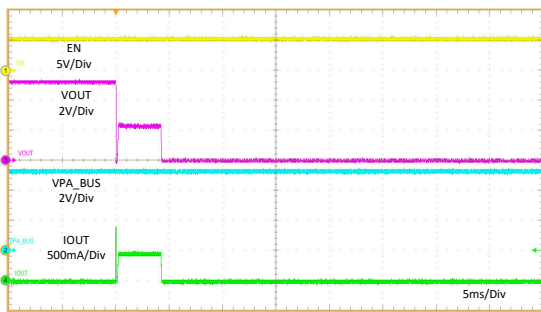
Figure 11-28. OUT short to 5.1-Ω Load
