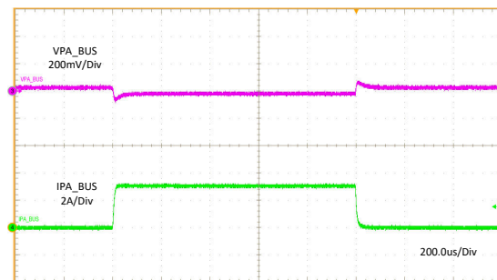
Figure 11-5. Load Regulation
