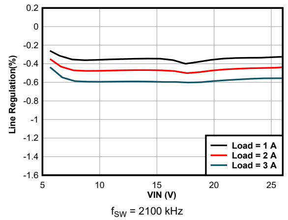
Figure 11-7. Line Regulation
