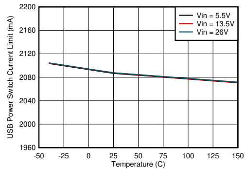
Figure 8-12. USB Power Switch Current Limit vs Junction Temperature R_{ILIM} = 15.4\text{ k}\Omega
