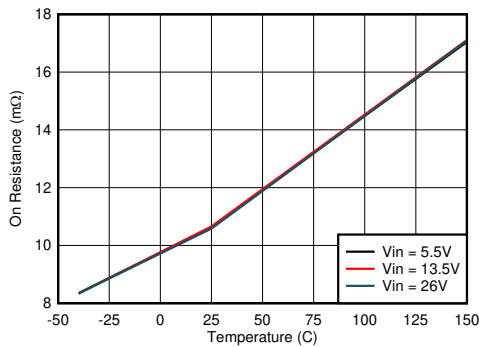
Figure 8-9. Low-side MOSFET on Resistance vs Junction Temperature I_{BUS} = 3\text{ A}
