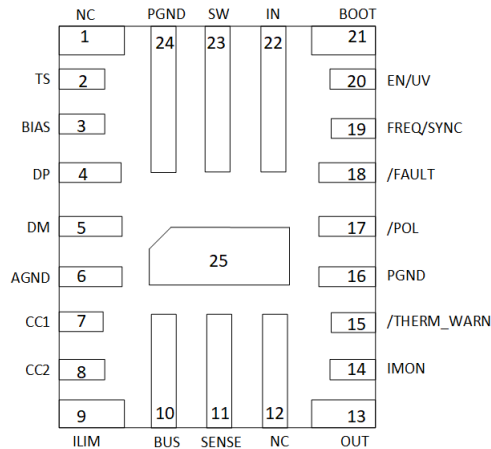
Figure 7-1. TPS2585x-Q1 RPQ Package 25-Pin (QFN) Top View
