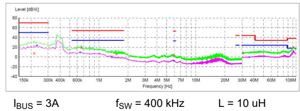
Figure 11-5. 400-KHz EMI Results (Without CM Filter)
