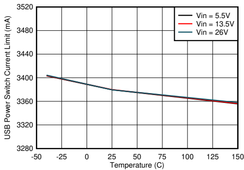
Figure 8-11. USB Power Switch Current Limit vs Junction Temperature R_{ILIM} = 9.53\text{ k}\Omega
