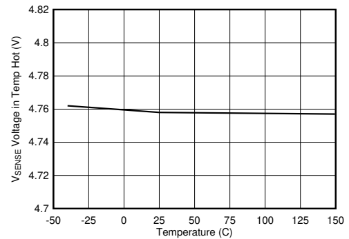
Figure 8-24. SENSE Voltage in Temperature Hot vs Junction Temperature
