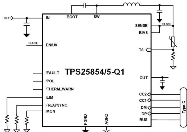
Simplified Schematic: TPS25854-Q1 and TPS25855-Q1
