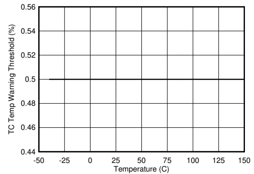
Figure 8-22. TS Temperature Warning Threshold vs Junction Temperature
