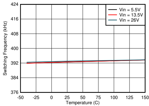
Figure 8-19. Switching Frequency vs Junction Temperature
