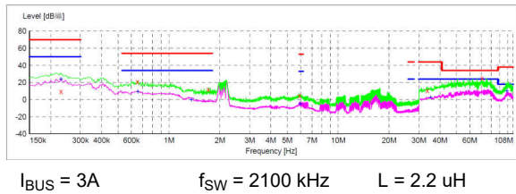
Figure 11-4. 2.1-MHz EMI Results (Without CM Filter)
