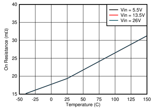
Figure 8-8. High-side MOSFET on Resistance vs Junction Temperature I_{BUS} = 3\text{ A}
