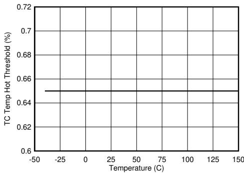
Figure 8-23. TS Temperature Hot Threshold vs Junction Temperature
