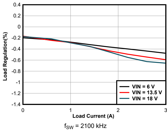
Figure 11-6. Load Regulation
