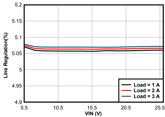
Figure 11-12. Dropout Characteristic
