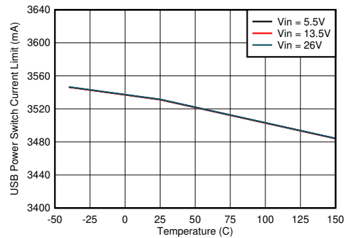
Figure 8-10. USB Power Switch Current Limit vs Junction Temperature ILIM = GND
