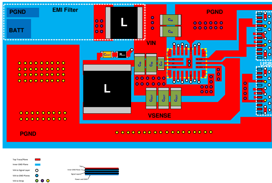
Figure 13-1. Layout Example
