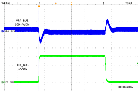
Figure 11-5. Load Regulation
