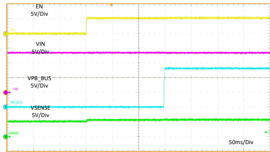
EN = 0\text{ V to }5\text{ V} PB\_CC1 = R_d I_{PB\_BUS} = 3\text{ A} Figure 11-18. Startup Relate to EN
