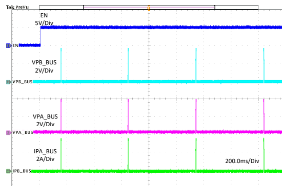
Figure 11-24. Enable Into 1- \Omega Load
