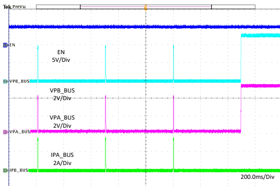
Figure 11-25. 1- \Omega Load Recovery
