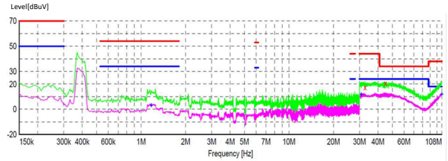
Figure 11-4. 400-kHz EMI Results (Without CM Filter)
