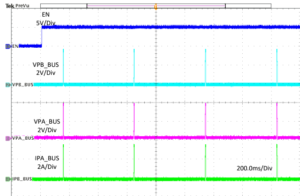
Figure 11-22. Enable Into Short
