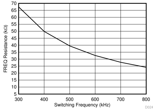
Figure 10-3. FREQ Set Resistor vs Switching Frequency
