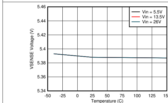
Figure 8-5. V_{SENSE} Voltage vs Junction Temperature
