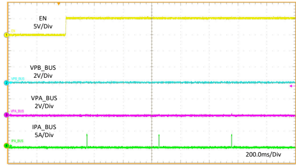
Figure 11-22. Enable Into Short
