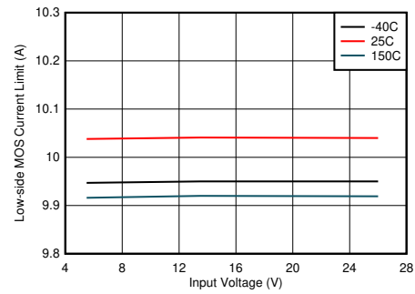
Figure 8-8. Low-side Current Limit vs Input Voltage
