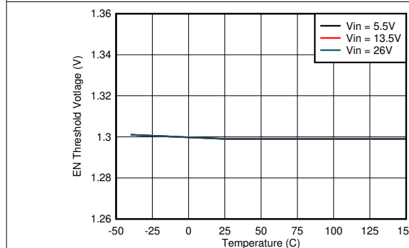
Figure 8-3. Precision Device Enable Threshold
