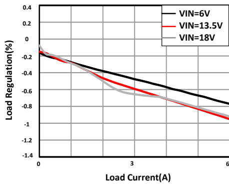
Figure 11-5. Load Regulation
