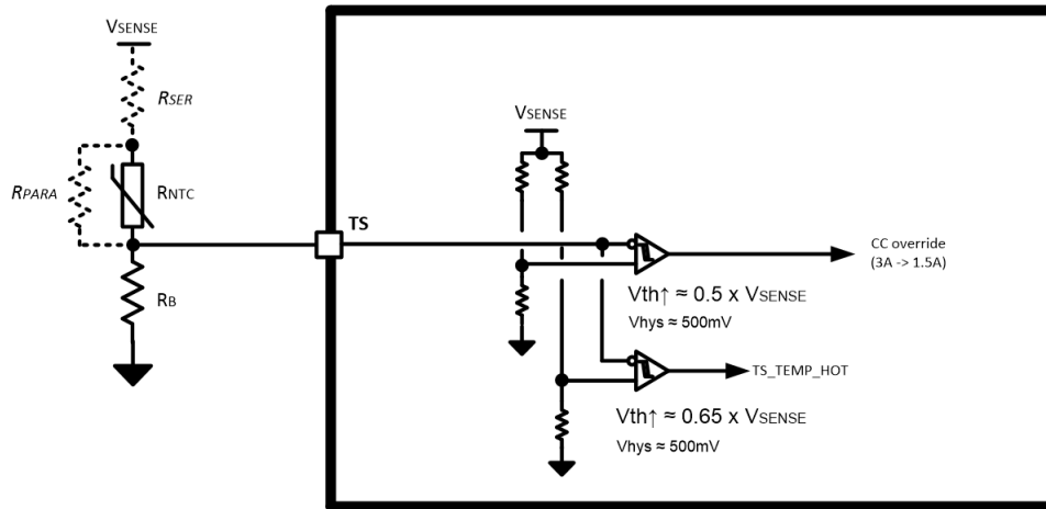
Figure 10-10. TS Input
