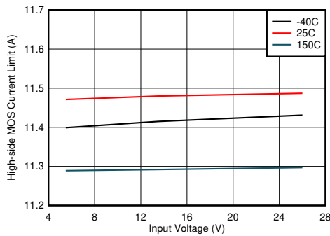
Figure 8-7. High-side Current Limit vs Input Voltage
