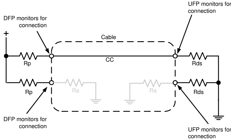
Figure 10-14. DFP-UFP Connection
