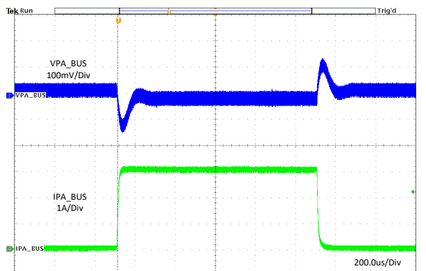
Figure 11-5. Load Regulation
