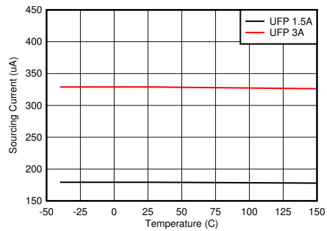
Figure 8-22. CC Sourcing Current vs Junction Temperature
