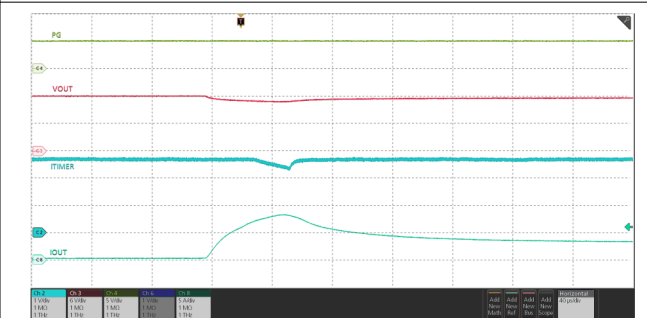
Figure 7-40. Active Current Limit Response – TPS25970x
