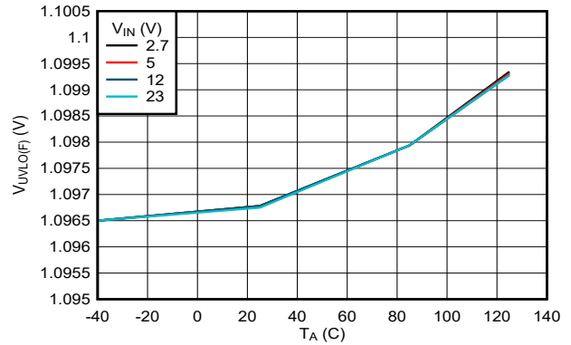
Figure 7-8. EN/UVLO Falling Threshold vs Temperature
