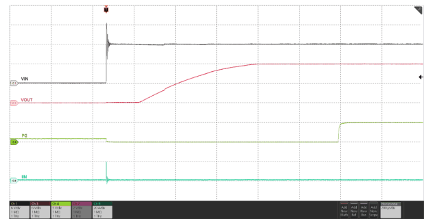
Figure 7-32. Input Hot-Plug
