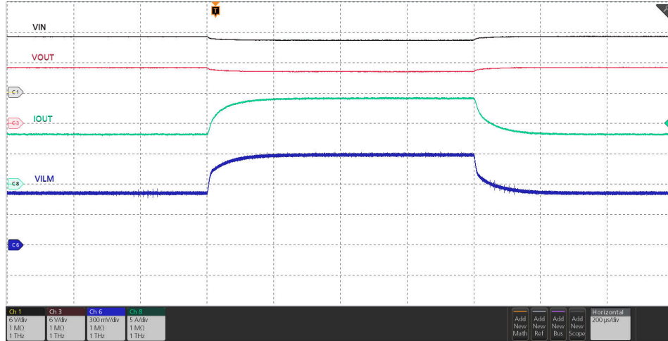
Figure 8-6. Analog Load Current Monitor Response
