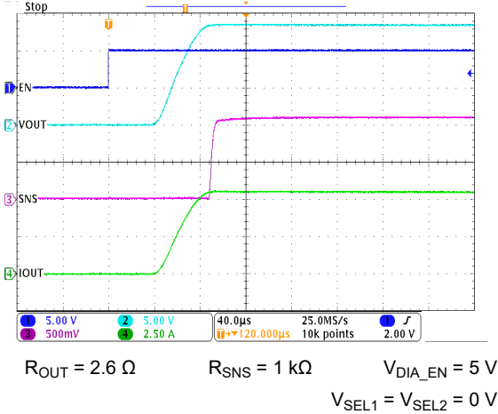
Figure 7-27. Turn-on Time ( t_{ON} )
