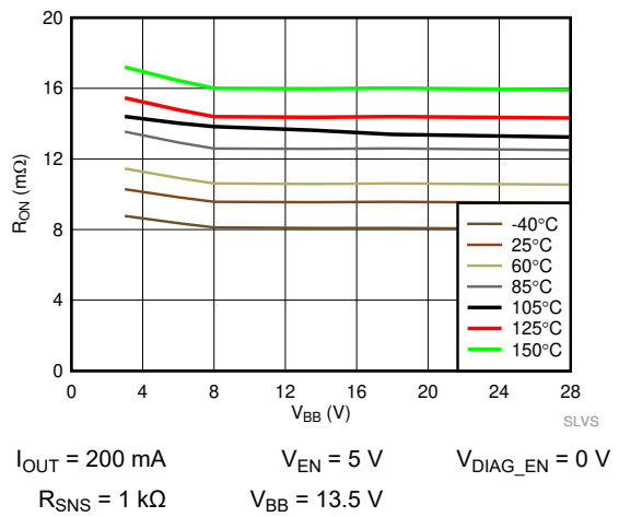
Figure 7-6. On Resistance ( R_{ON} ) vs V_{BB}
