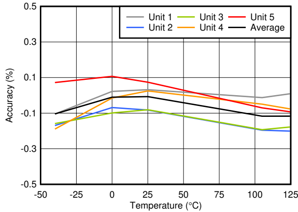
TPS3851G50, V_{ITN} = 4.8\text{ V}
