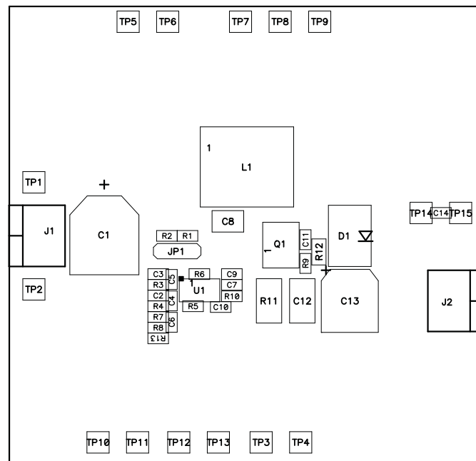
Figure 37. Component Placement
