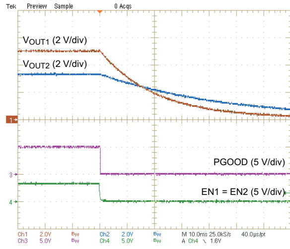
Figure 24. Output Discharge
