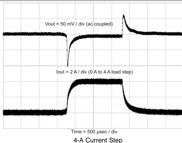
Figure 41. Transient Response
