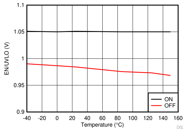
Figure 6-15. EN/UVLO Thresholds vs Junction Temperature
