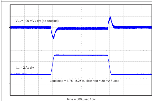
Figure 8-4. Transient Response, 3.5 A Step
