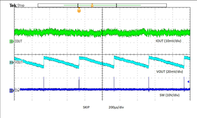
Figure 6-18. V_{OUT} Ripple, Skip Mode, 10-mA Load
