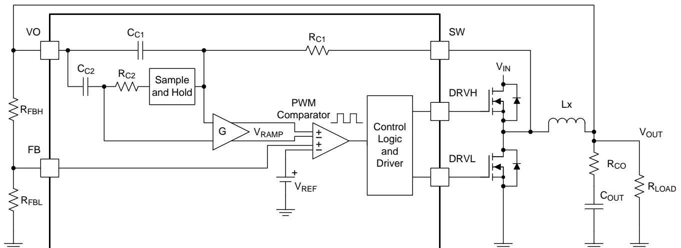
Figure 32. D-CAP3 Mode
