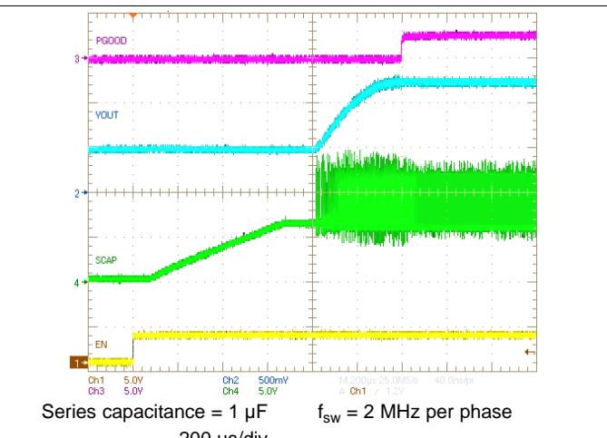
Figure 30. Pre-biased Startup Through EN
