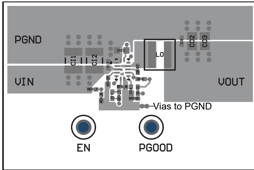
Figure 10-1. Top Layer Layout
