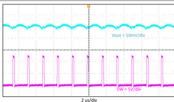
Figure 8-7. Output Voltage Ripple, I_{out} = 3 A
