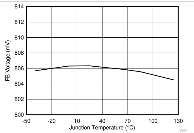
Figure 7-2. FB Voltage vs Junction Temperature
