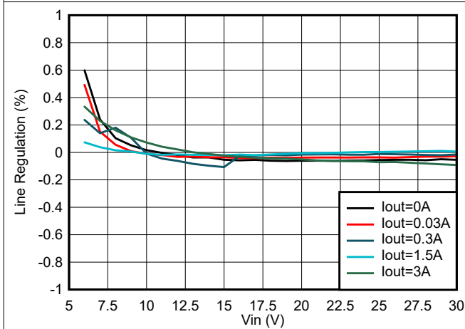
Figure 8-4. Line Regulation
