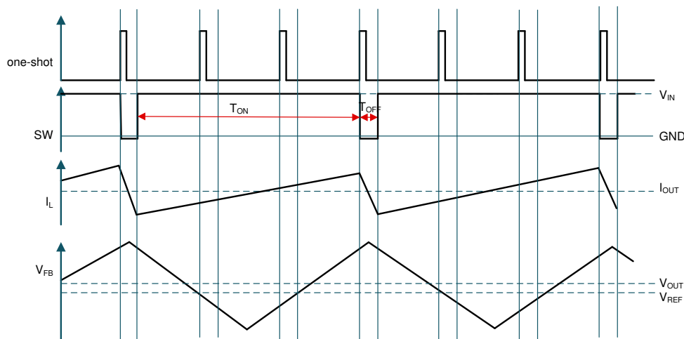
Figure 5. Two-times On-Time Extension ( V_{IN} / V_{OUT} \leq 1.2 \text{ V} )
