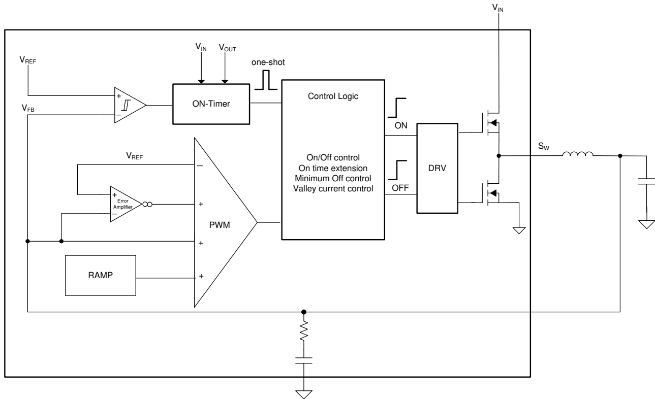
Figure 2. Detail D-CAP3™ Control Block Diagram in TPS568230
