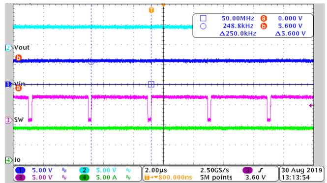
Figure 9. One-time On-Time Extension
