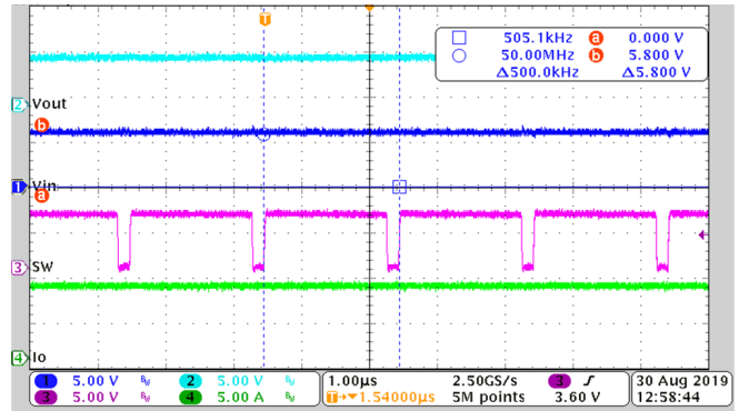
Figure 7. Normal Operation When F_{sw} Drops to 500 kHz
