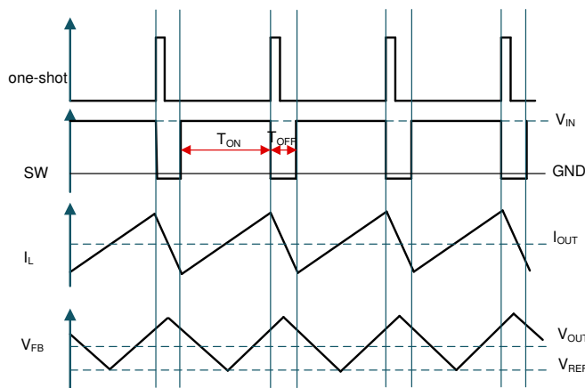
Figure 3. Normal Operation Without On-Time Extension
