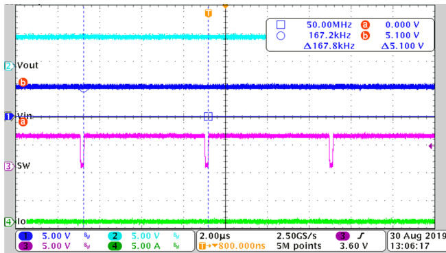
Figure 10. Two-times On-Time Extension
