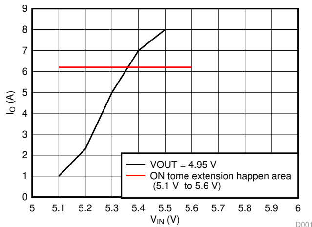
Figure 12. TPS568230 V_{IN} vs I_O Curve
