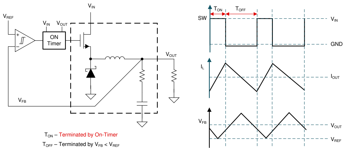
Figure 1. Adaptive On-Time Control (AOT Control)
