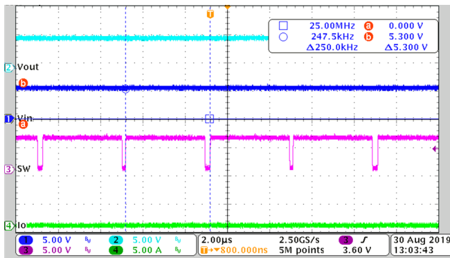
Figure 8. One-time On-Time Extension
