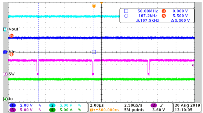
Figure 11. Two-times On-Time Extension
