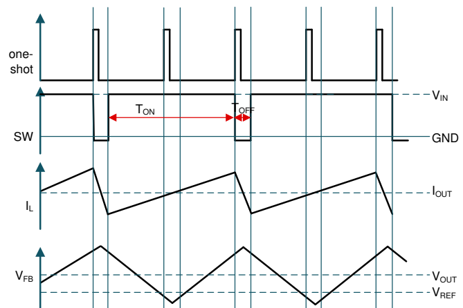
Figure 4. One-time On-Time Extension ( 1.2 \text{ V} < V_{IN} / V_{OUT} \leq 1.6 \text{ V} )
