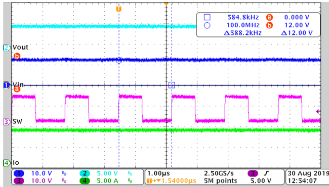
Figure 6. Normal Operation Without On-Time Extension
