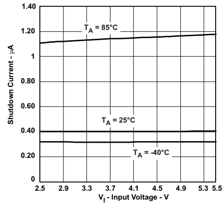
Figure 13. Shutdown Current vs Input Voltage
