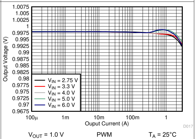
Figure 10-19. Output Voltage vs Output Current
