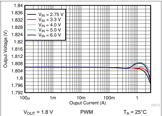
Figure 10-15. Output Voltage vs Output Current
