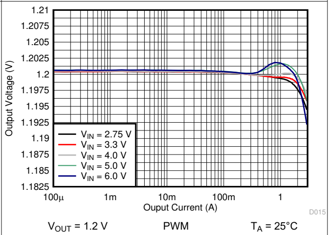
Figure 10-17. Output Voltage vs Output Current
