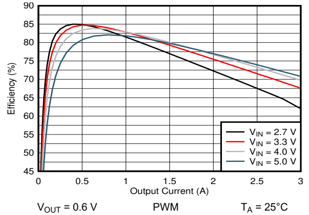
Figure 10-9. Efficiency Versus Output Current
