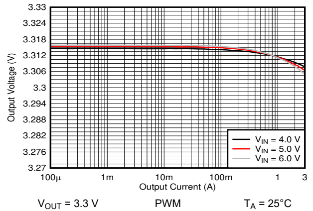
Figure 10-11. Output Voltage Versus Output Current
