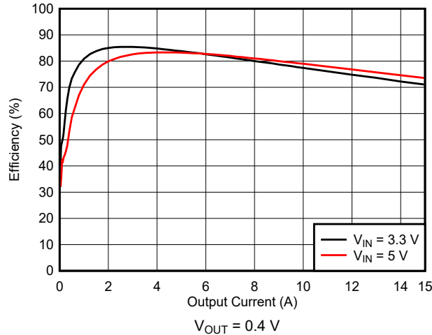
Figure 10-2. Efficiency
