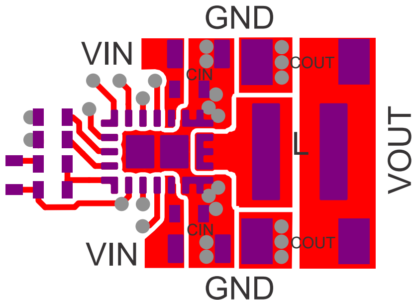
Figure 10-24. Layout Example
