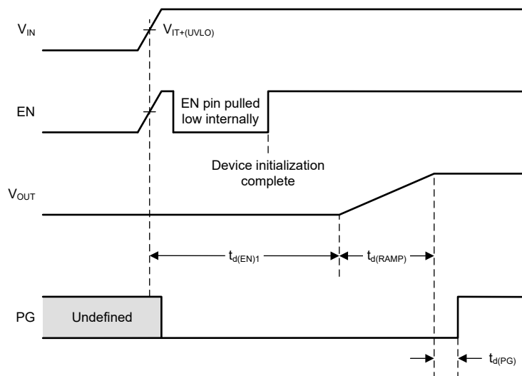
Figure 9-7. Start-Up Timing When EN is Pulled Up to V_{\text{IN}}
