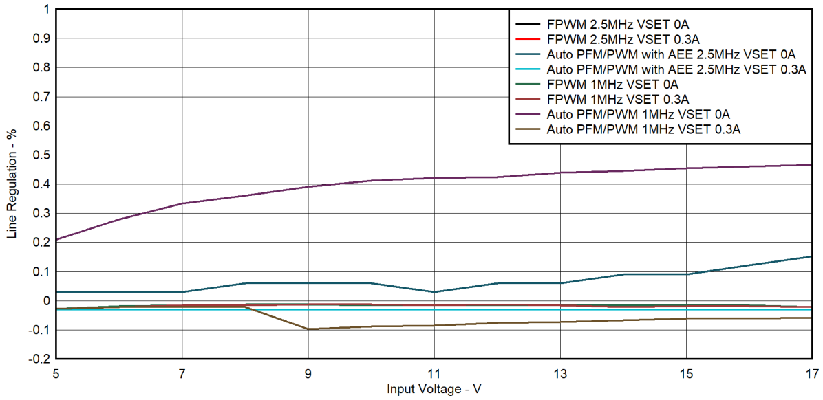
Figure 5-3. Line Regulation, V_{IN} = 5\text{ V}–17\text{ V} , V_{OUT} = 3.3\text{ V} , I_{OUT} = 0\text{ A} and 300\text{ mA} , F_{SW} = 2.5\text{ MHz} and 1\text{ MHz}
