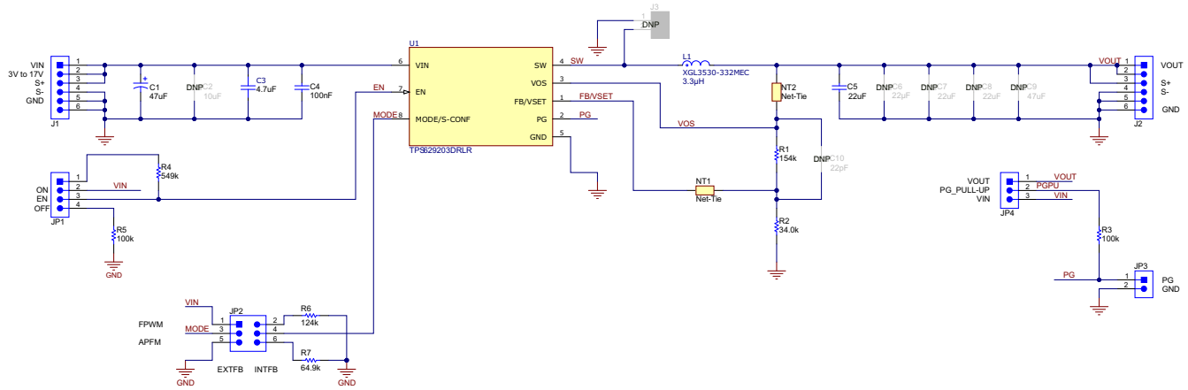
Figure 7-1. TPS629203EVM Schematic
