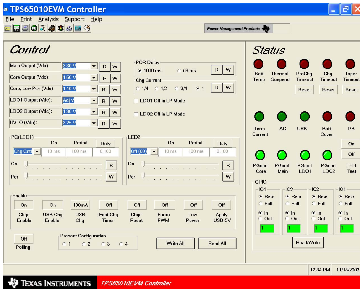
Figure 1. Main Control Window
