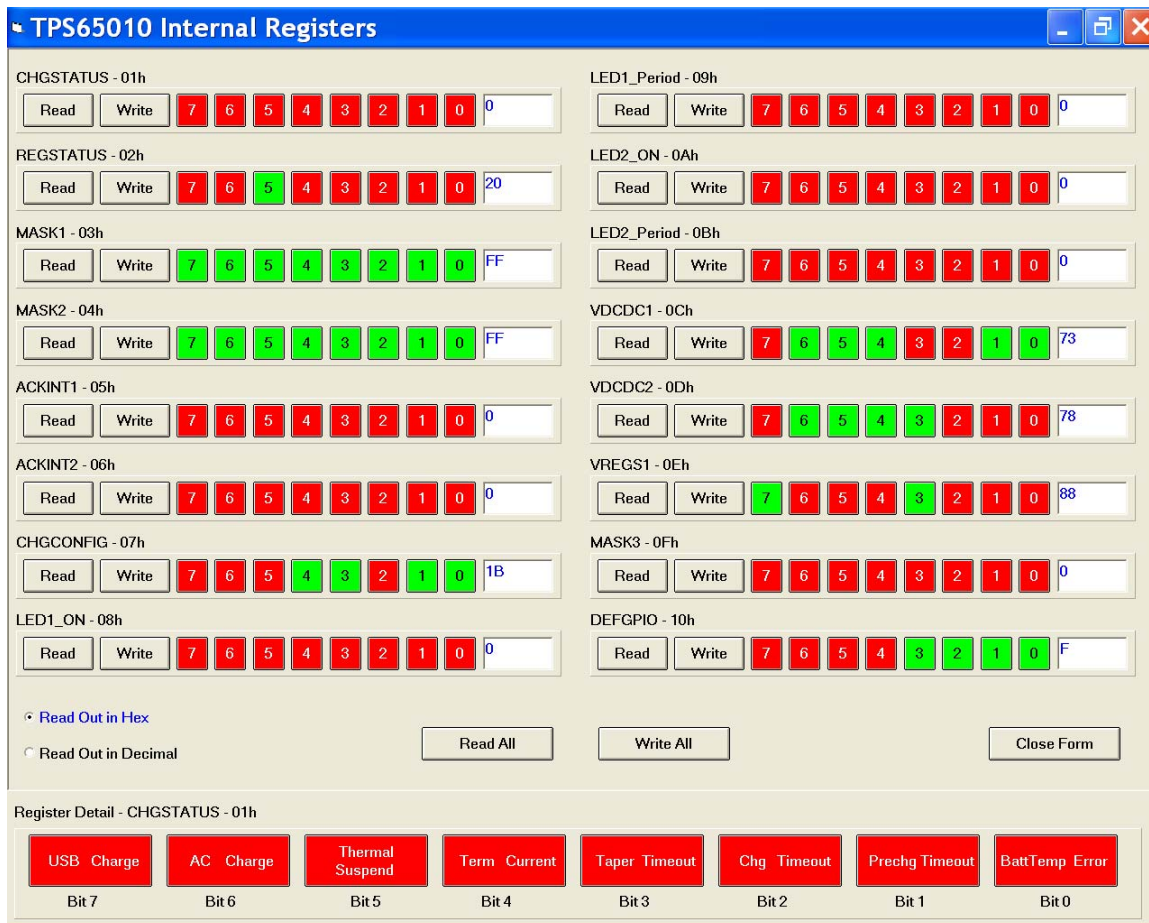
Figure 2. Internal Registers Window
