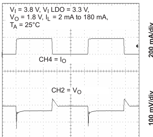
Figure 18. Load Transient Response (LDO2)
