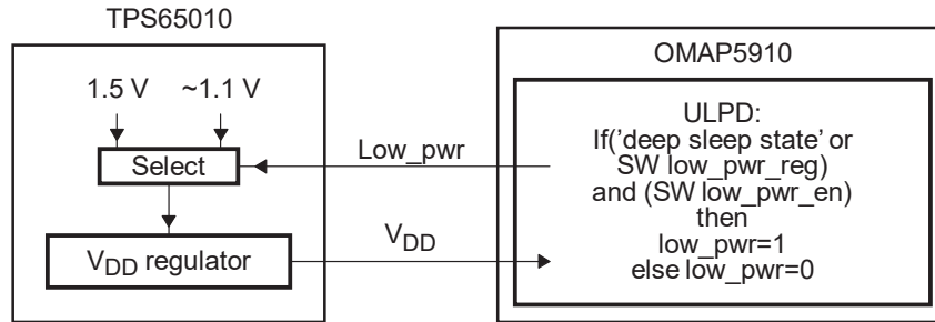
Figure 2. UPLD Characteristics
