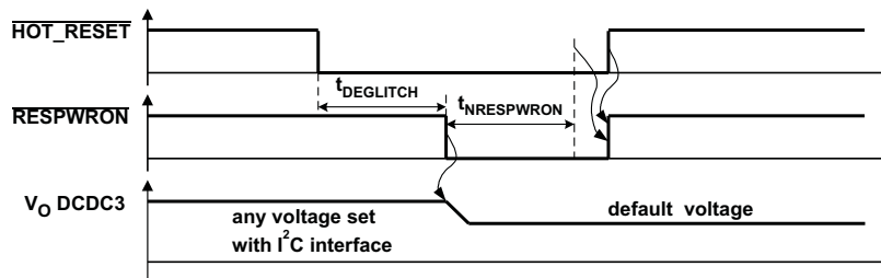
Figure 1. HOT_RESET Timing
