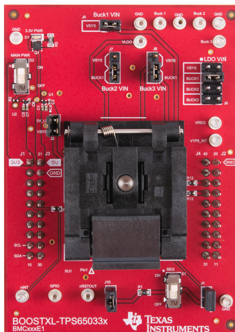
Figure 1. TPS650330-Q1 Programming BoosterPack™ EVM
