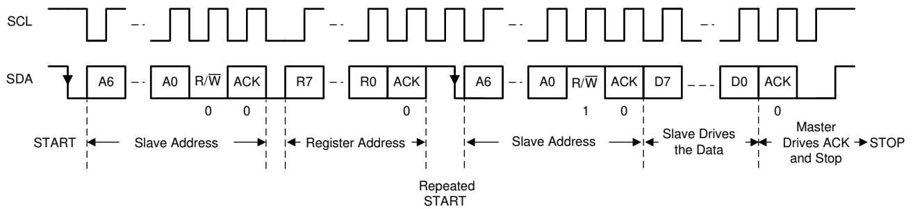
Figure 8-33. I 2 C Interface READ from TPS650864 in F/S Mode (Only Repeated START is Supported)
