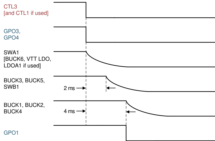
Figure 8-5. TPS6508640 Power-Down Sequence
