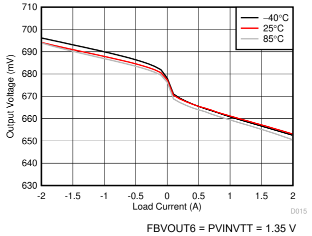
Figure 7-8. VTT LDO Regulation
