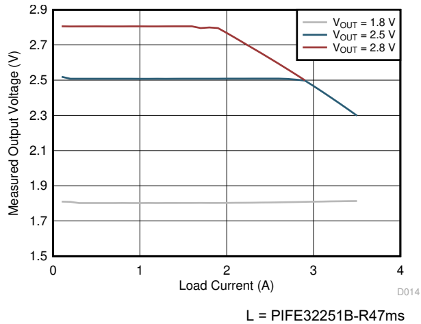
Figure 7-7. Converter Load Current Limitations with V_{IN} = 3.3\text{ V}
