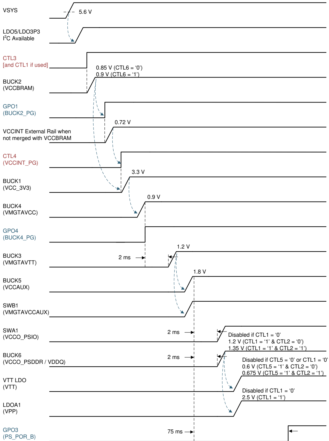
Figure 8-4. TPS6508640 Power-Up Sequence
