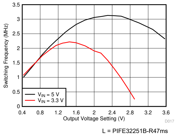
Figure 7-10. Converter Switching Frequency (25-mV Step Size)
