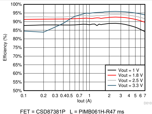
Figure 9-8. BUCK1 Efficiency at V IN = 5 V
