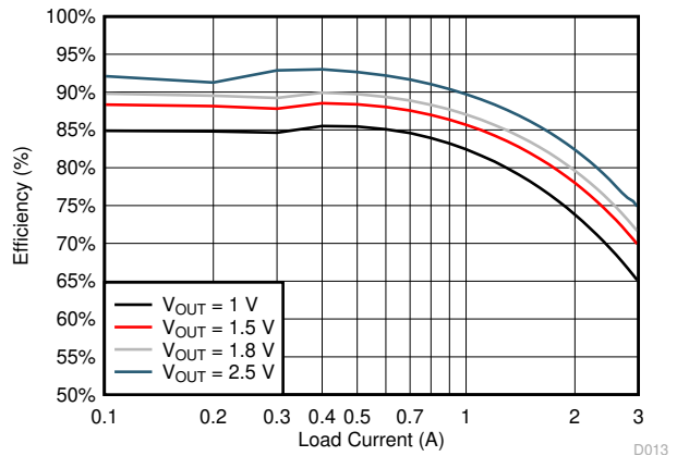
Figure 7-4. Example BUCK1 Efficiency at V IN = 18 V
