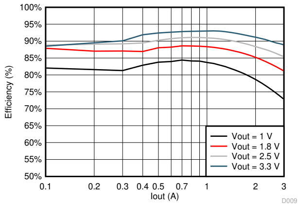
Figure 7-3. Example BUCK1 Efficiency at V IN = 13 V
