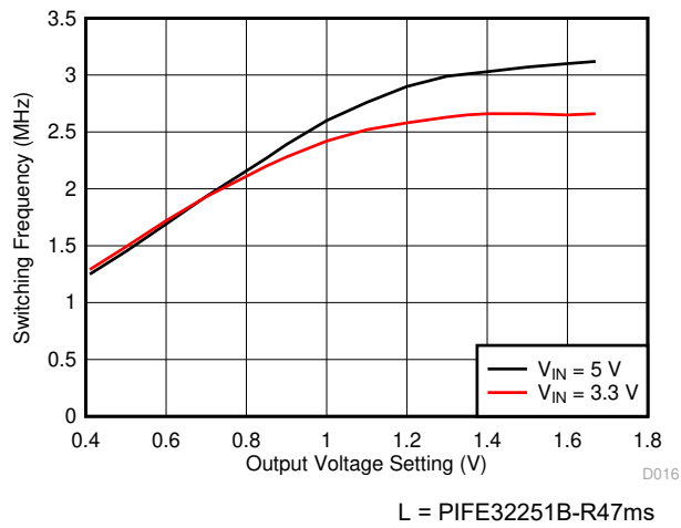
Figure 7-9. Converter Switching Frequency (10-mV Step Size)
