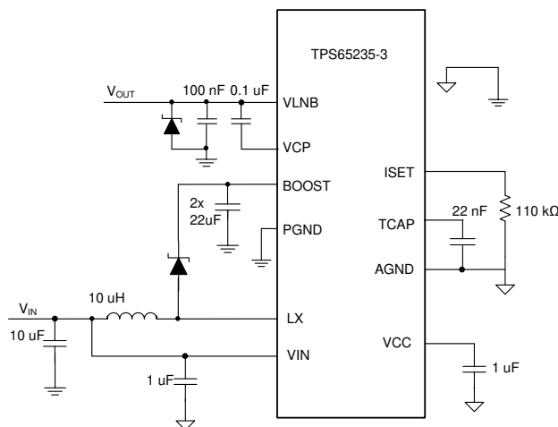
Simplified Schematic
