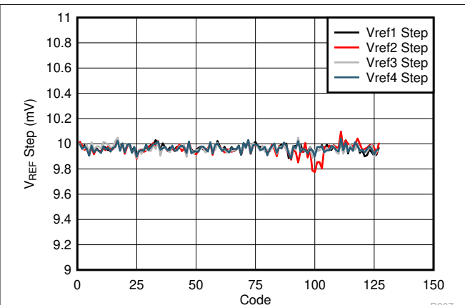
Figure 9-6. V REF Step Accuracy vs Code
