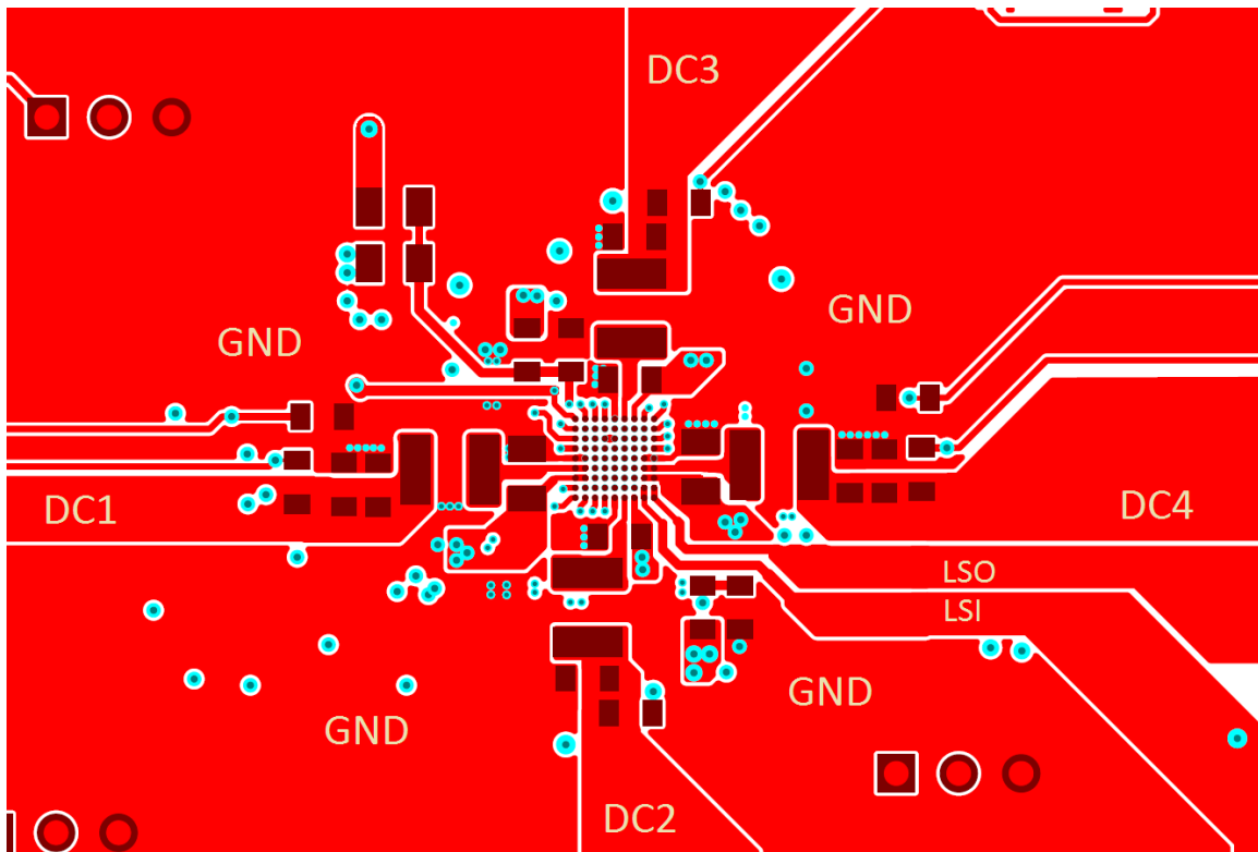
Figure 10-1. Layout Example
