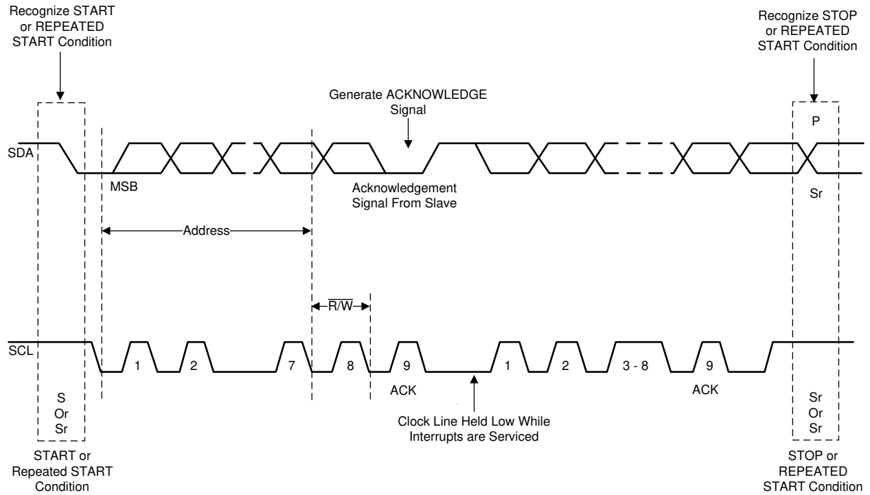
Figure 8-22. Bus Protocol
