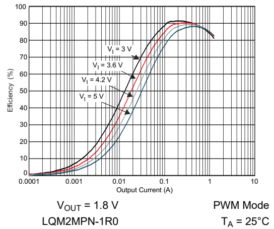
Figure 6-8. DCDC2 Efficiency vs Output Current
